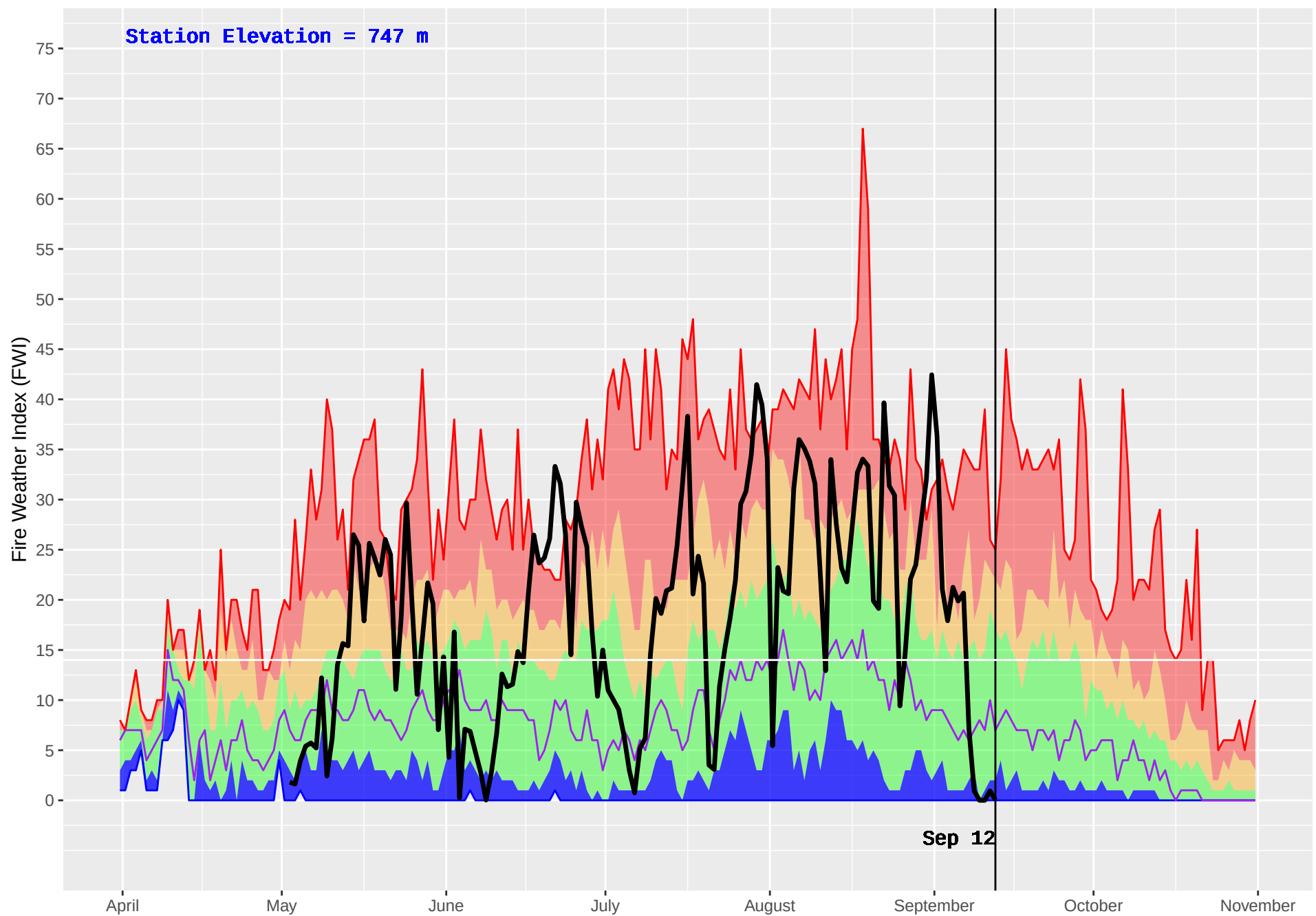
PEDEN (178) : Historical (1984–2016) and Current (2018) Daily Fire Weather Index (FWI)
