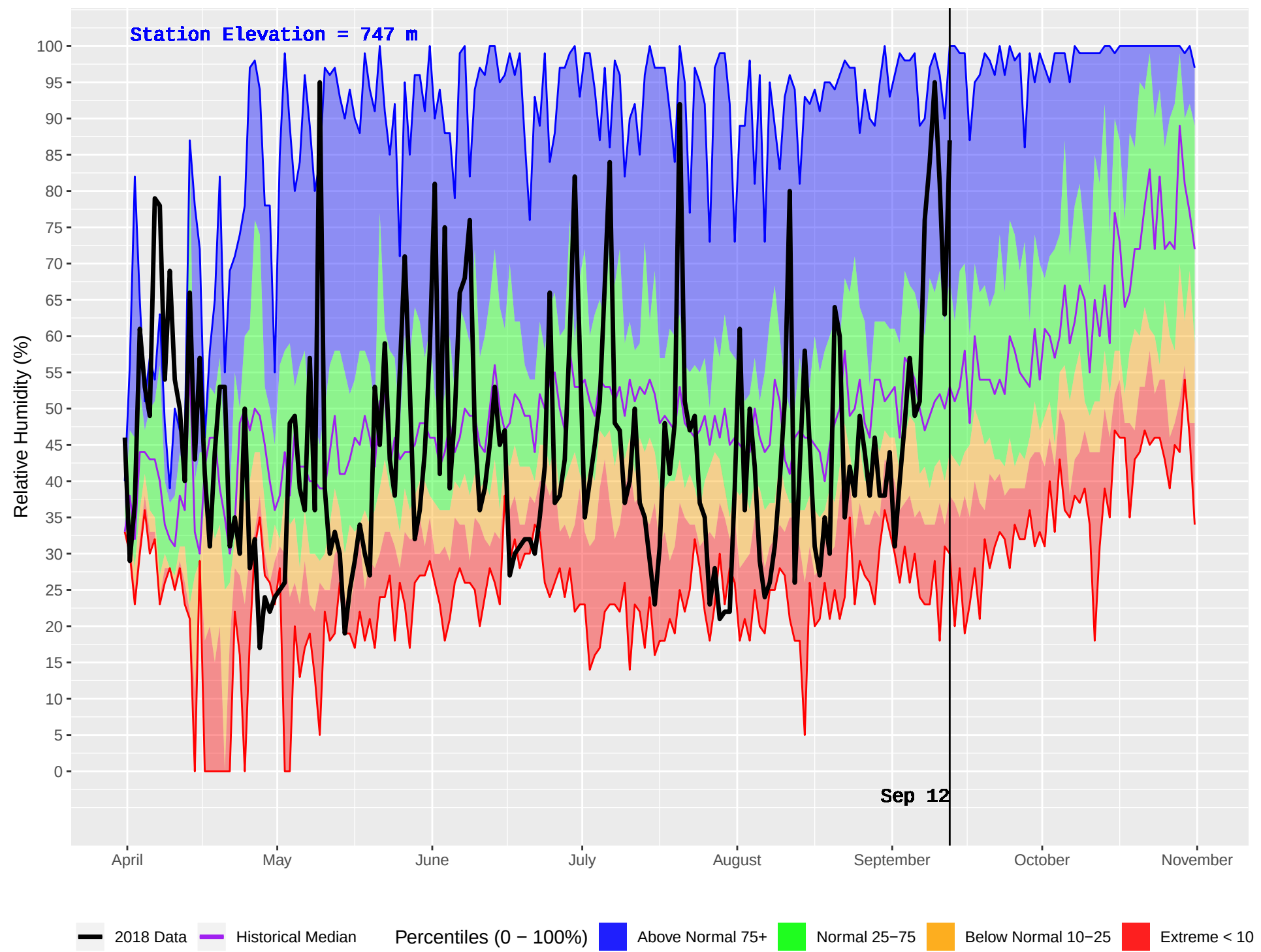
PEDEN (178) : Historical (1984–2016) and Current (2018) Daily Relative Humidity
