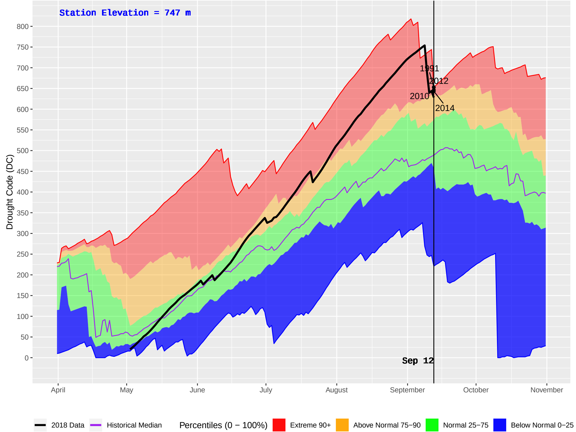
PEDEN (178) : Historical (1984–2016) and Current (2018) Daily Drought Code (DC)
