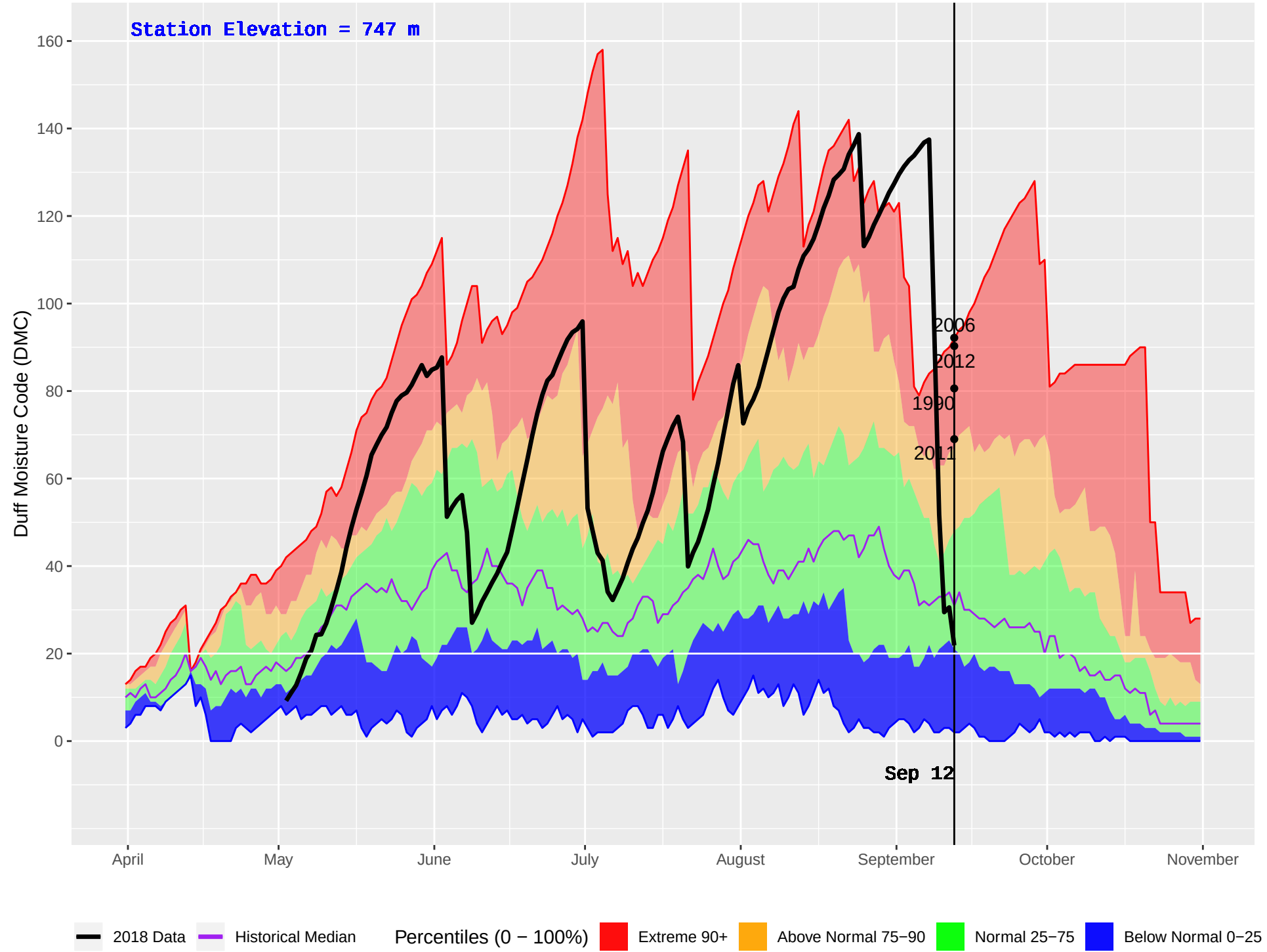
PEDEN (178) : Historical (1984–2016) and Current (2018) Daily Duff Moisture Code (DMC)
