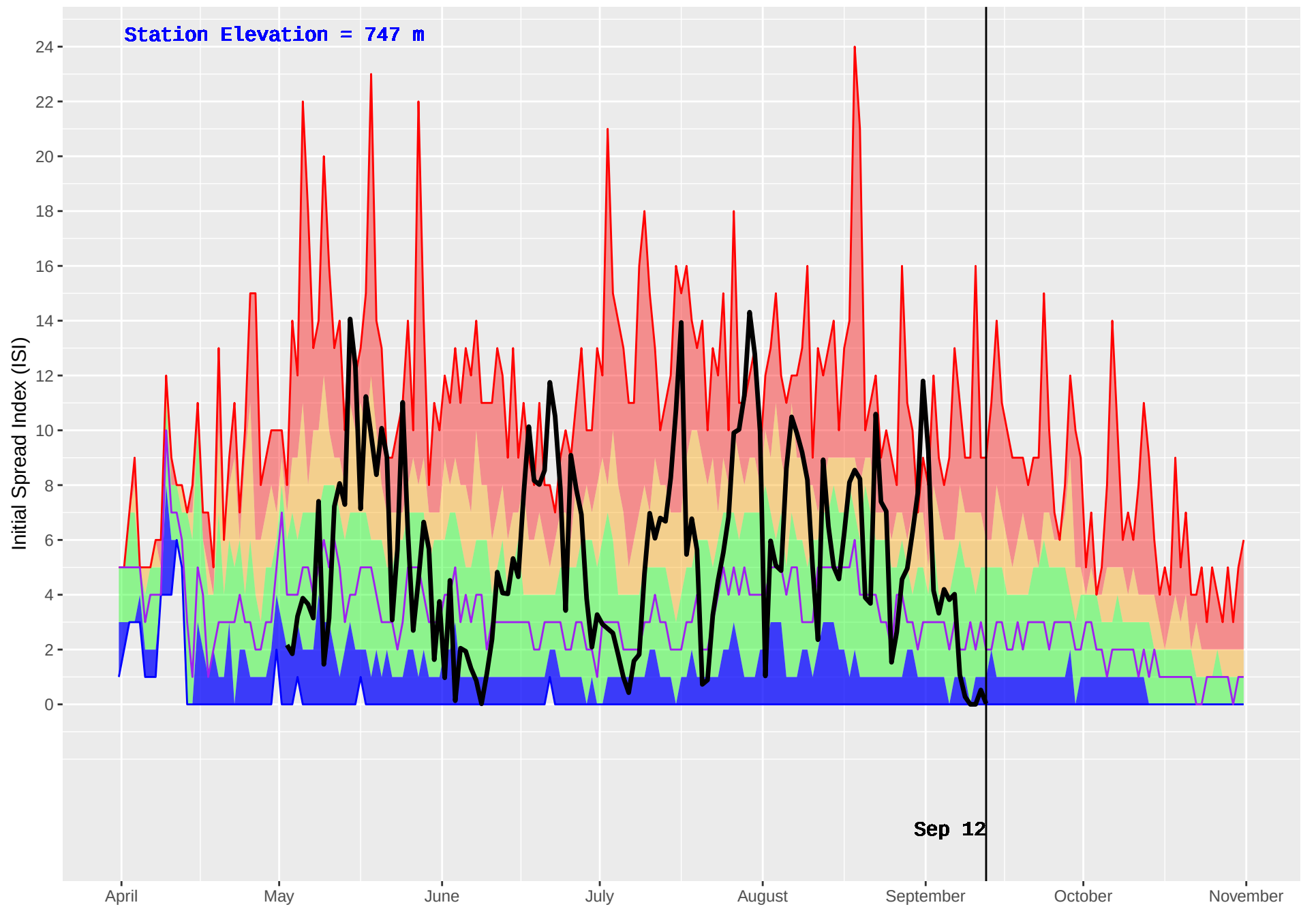
PEDEN (178) : Historical (1984–2016) and Current (2018) Daily Initial Spread Index (ISI)
