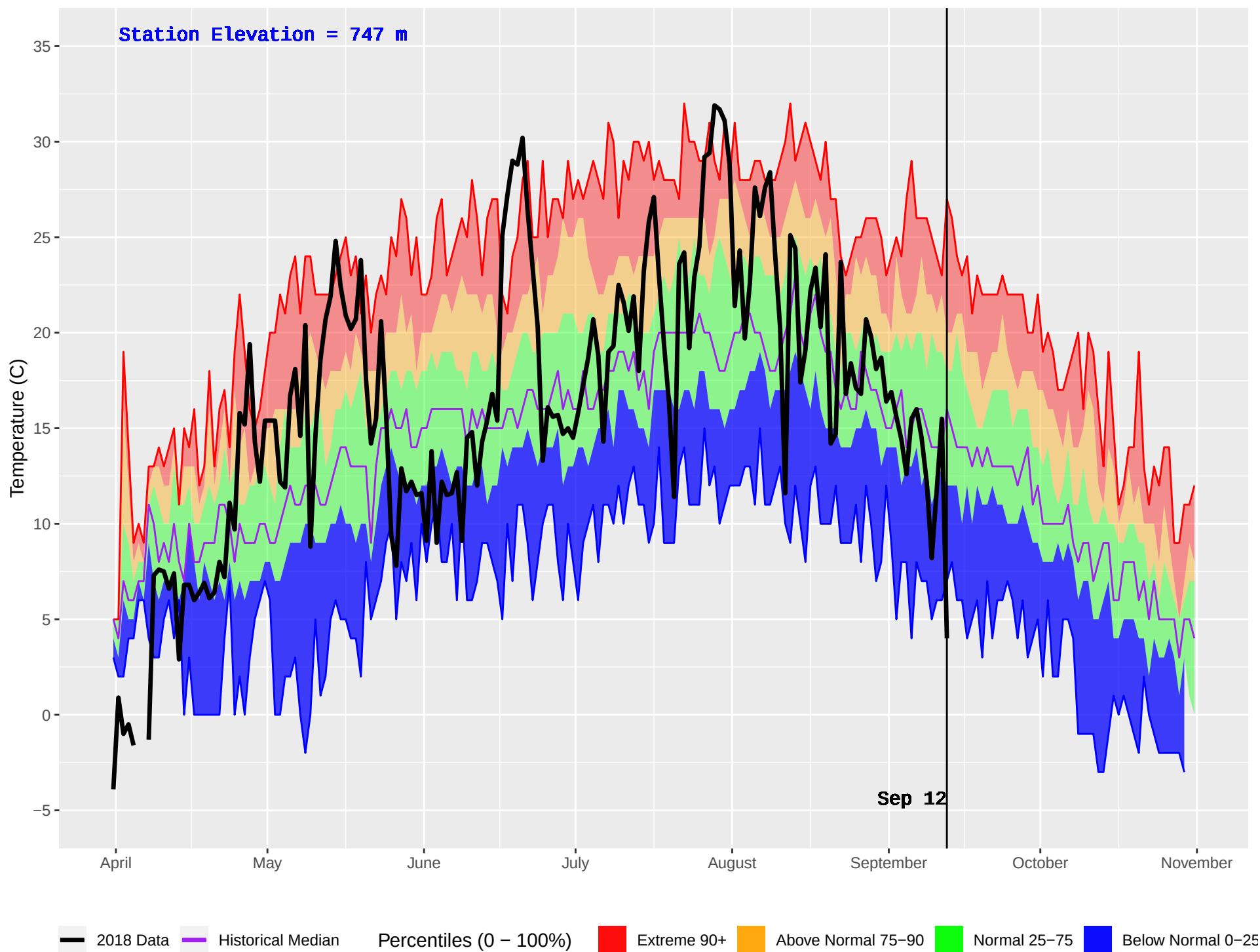
PEDEN (178) : Historical (1984–2016) and Current (2018) Daily Temperature
