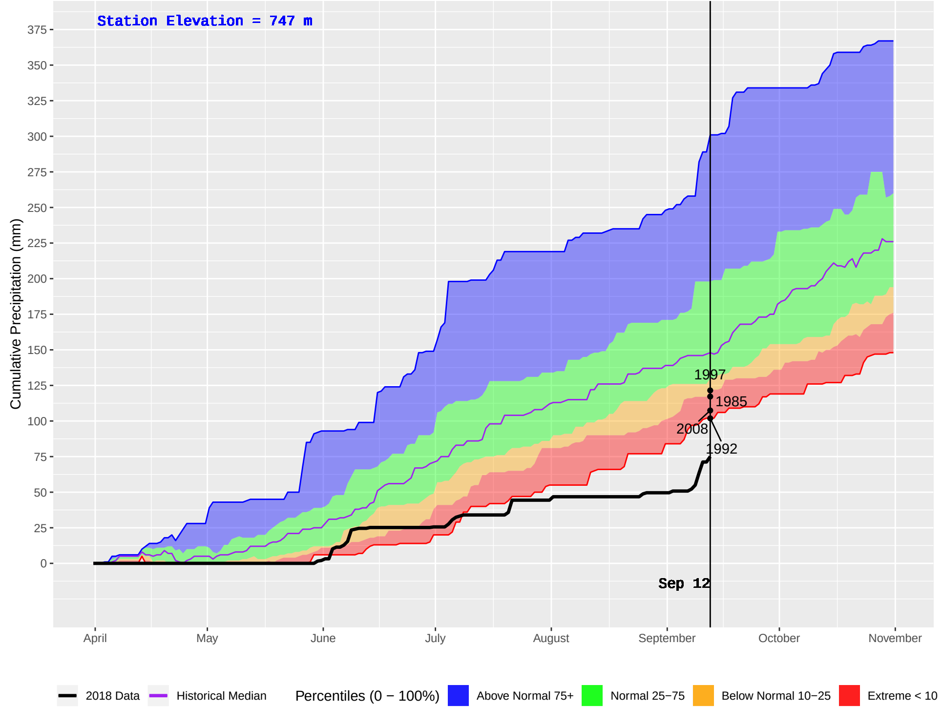
PEDEN (178) : Historical (1984–2016) and Current (2018) Daily Cumulative Precipitation
