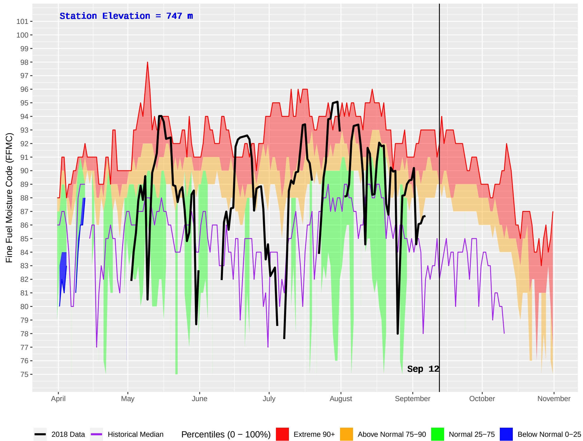
PEDEN (178) : Historical (1984–2016) and Current (2018) Daily Fine Fuel Moisture Code (FFMC)
