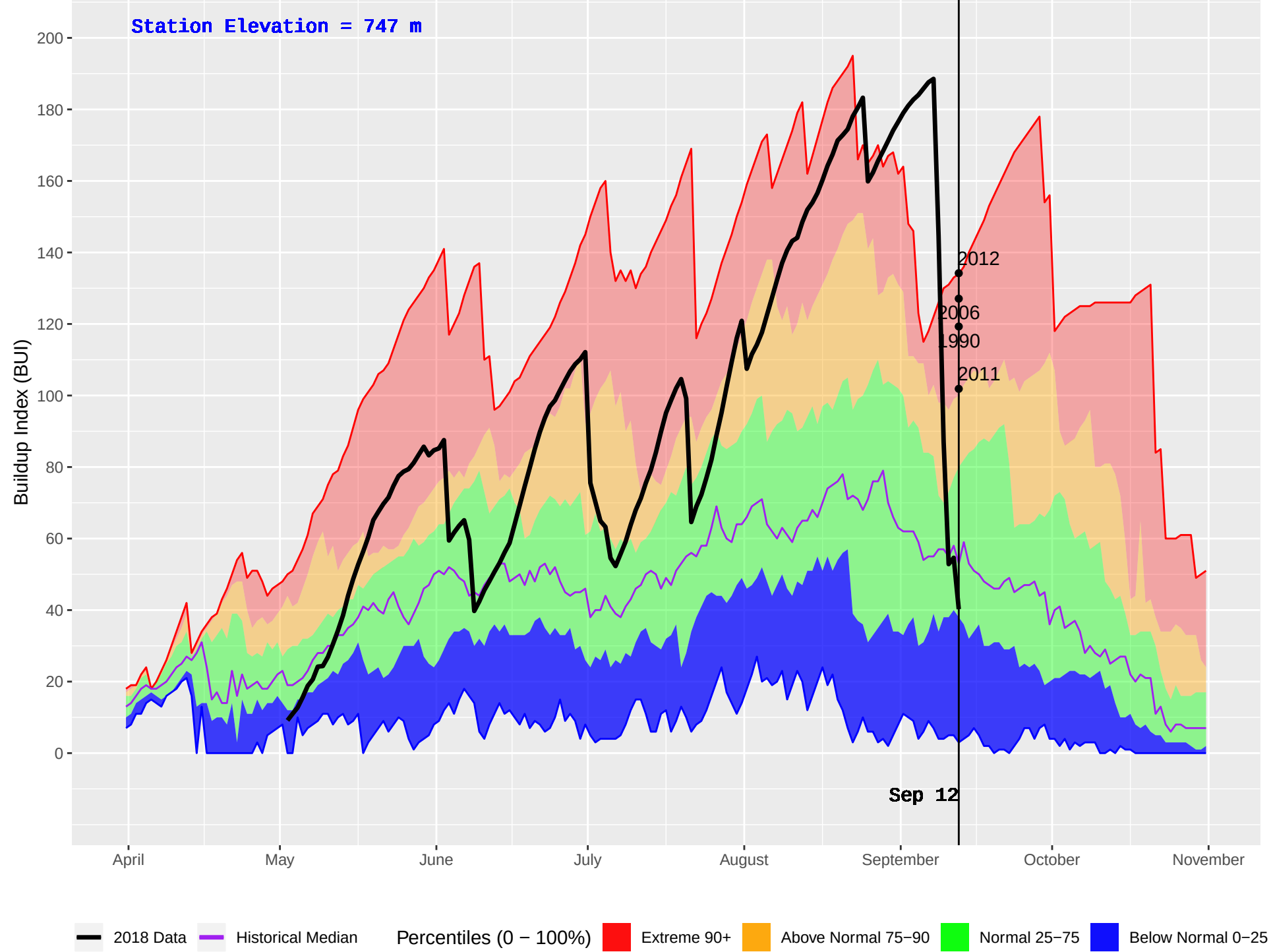
PEDEN (178) : Historical (1984–2016) and Current (2018) Daily Buildup Index (BUI)
